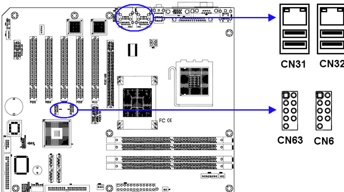
Figure 2.1: USB Ports
